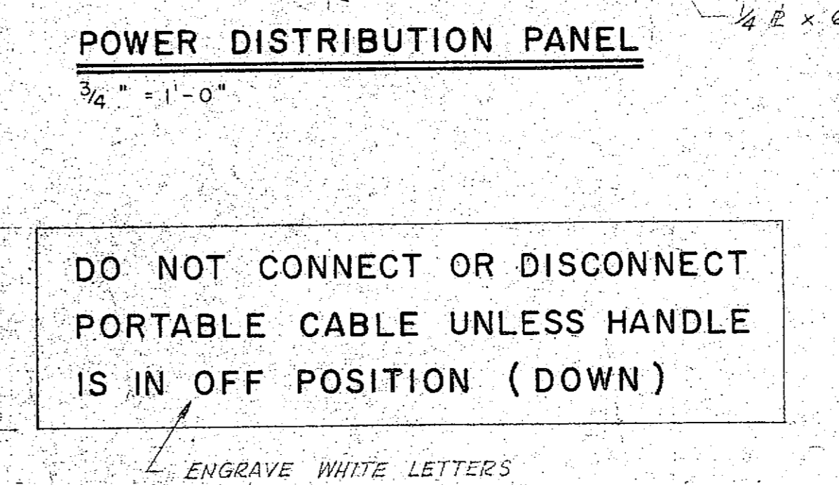
SIGN DETAIL
