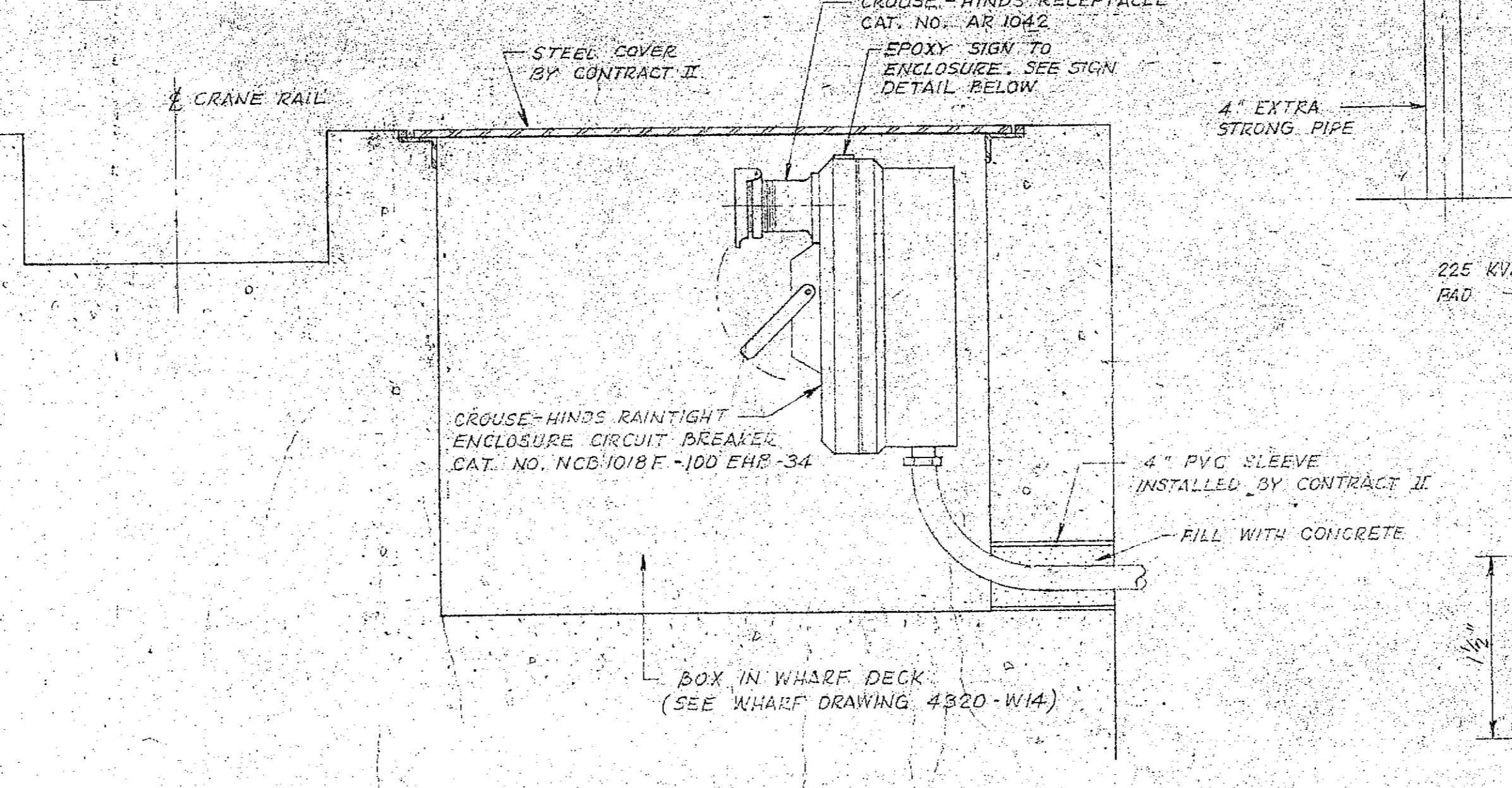
CRANE STANDBY POWER OUTLET
