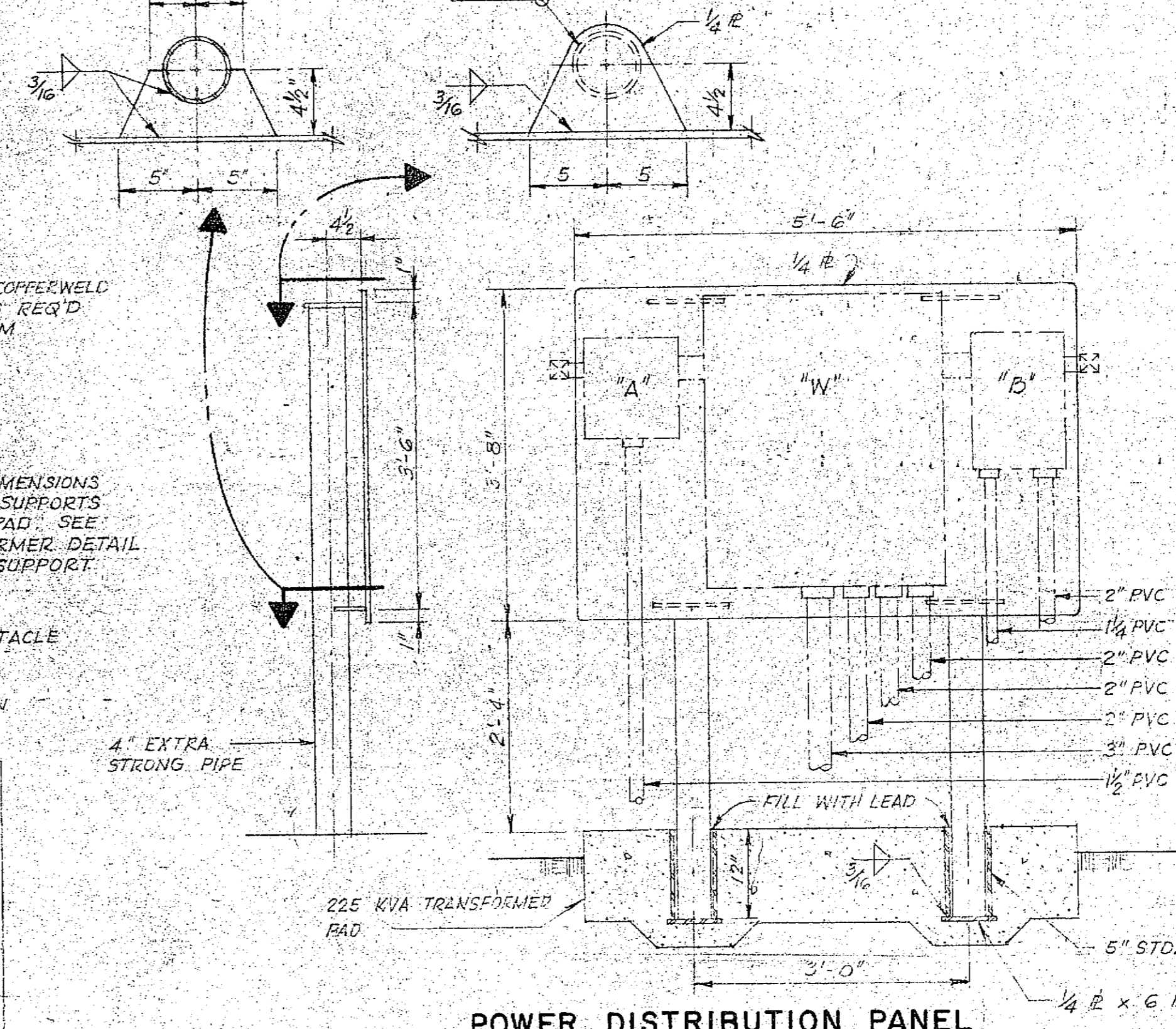
POWER DISTRIBUTION PANEL
