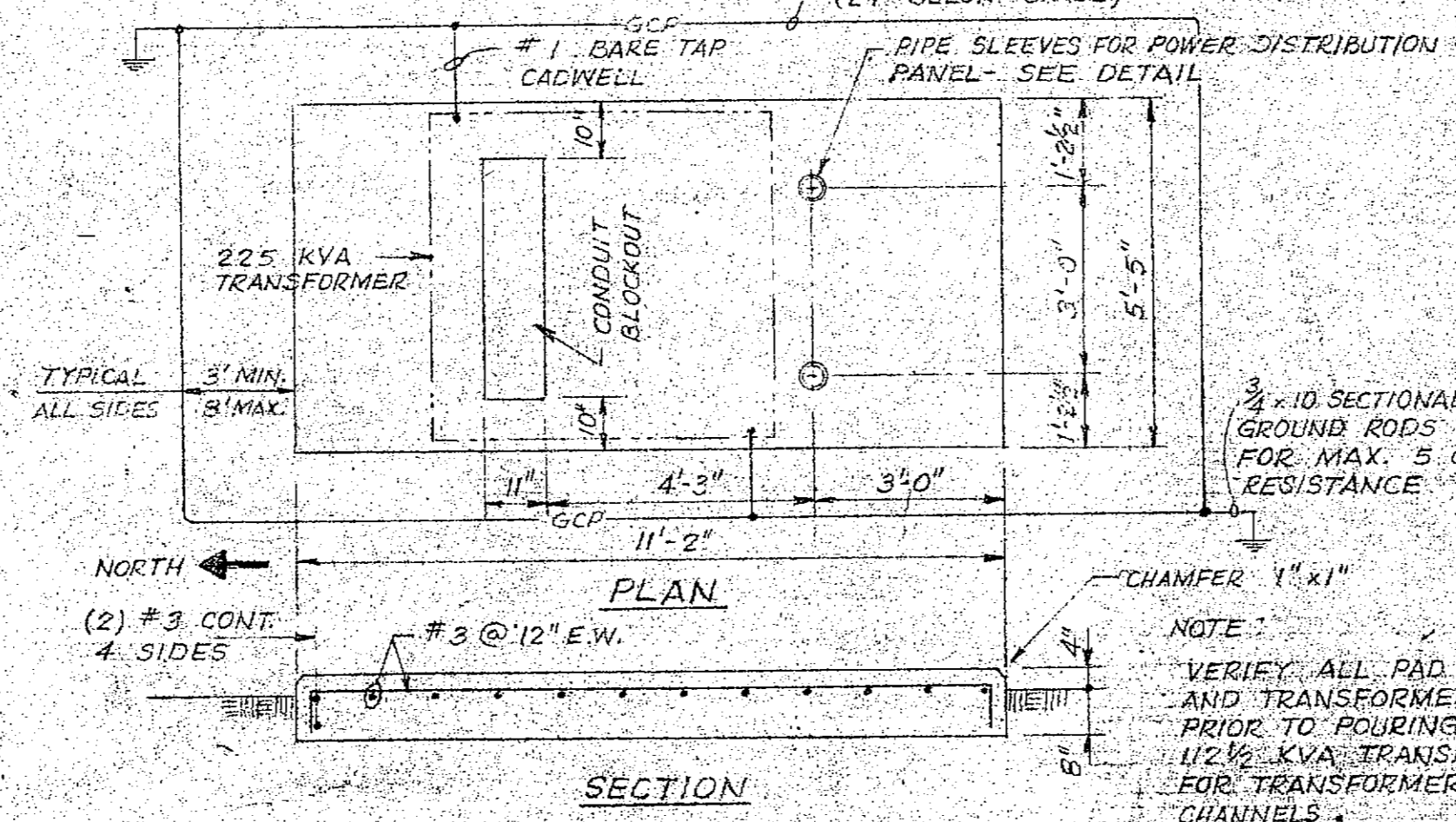
225 KVA TRANSFORMER PAD DETAIL
